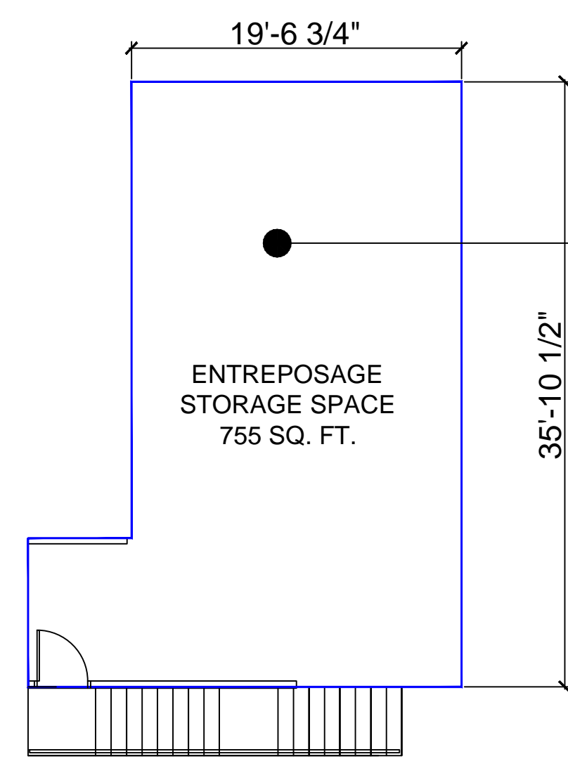
PLAN MEZZANINE
