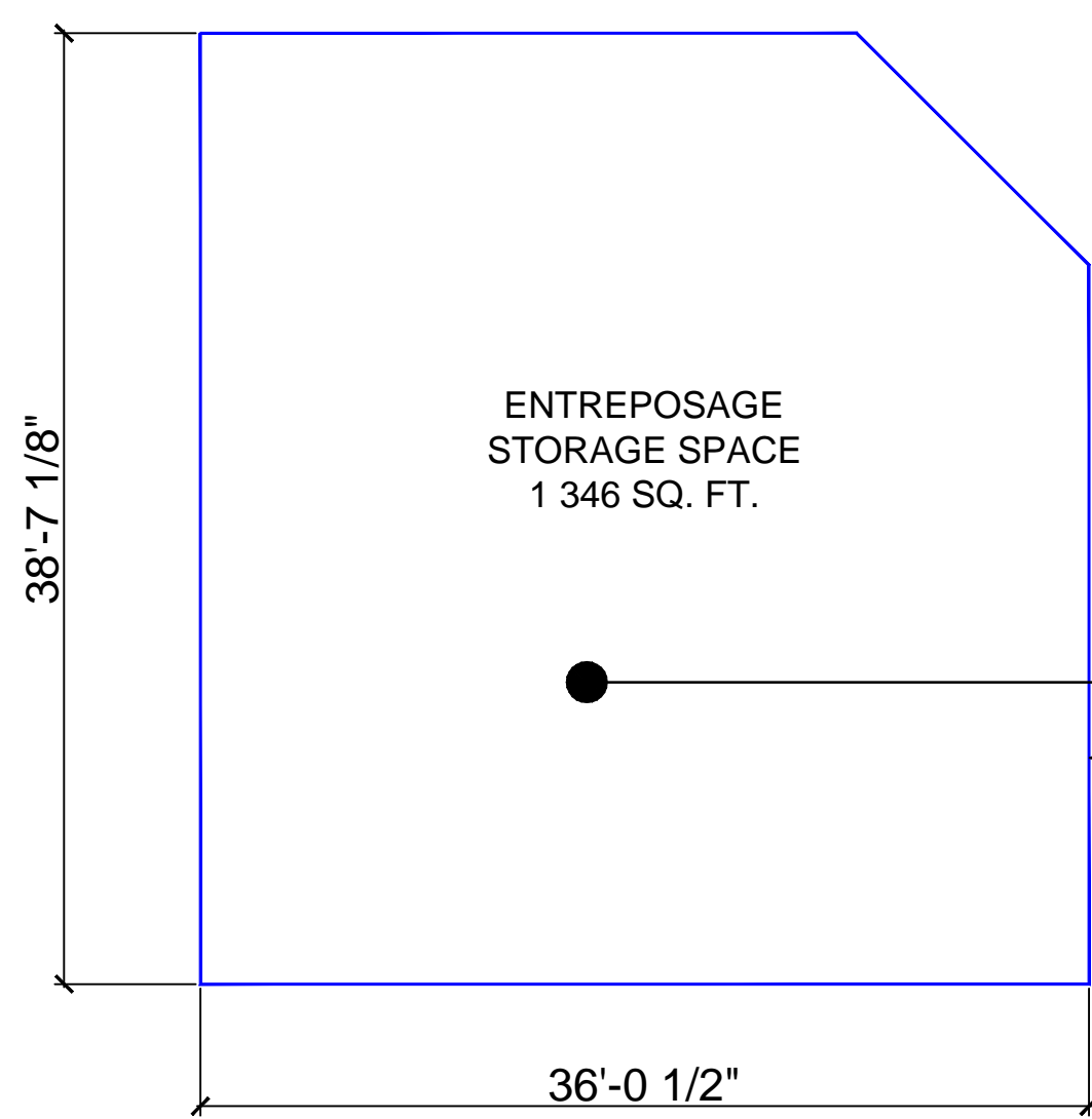
PLAN MEZZANINE
