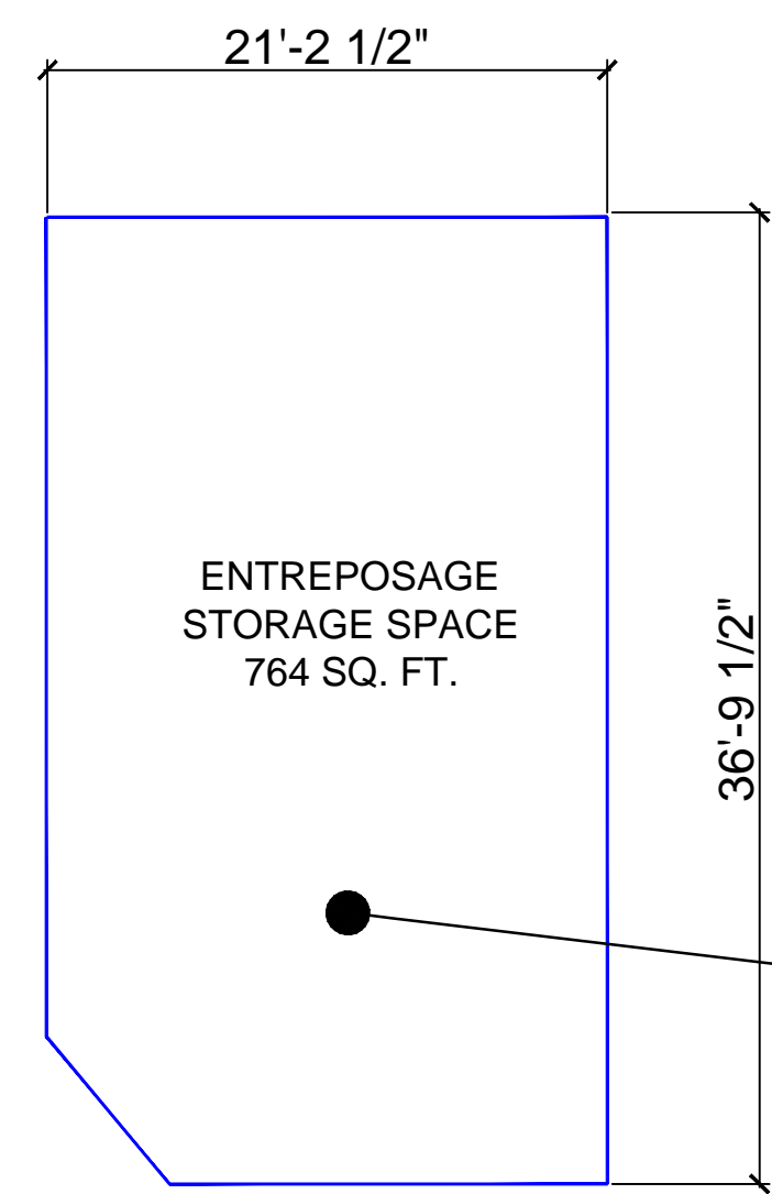
PLAN MEZZANINE
