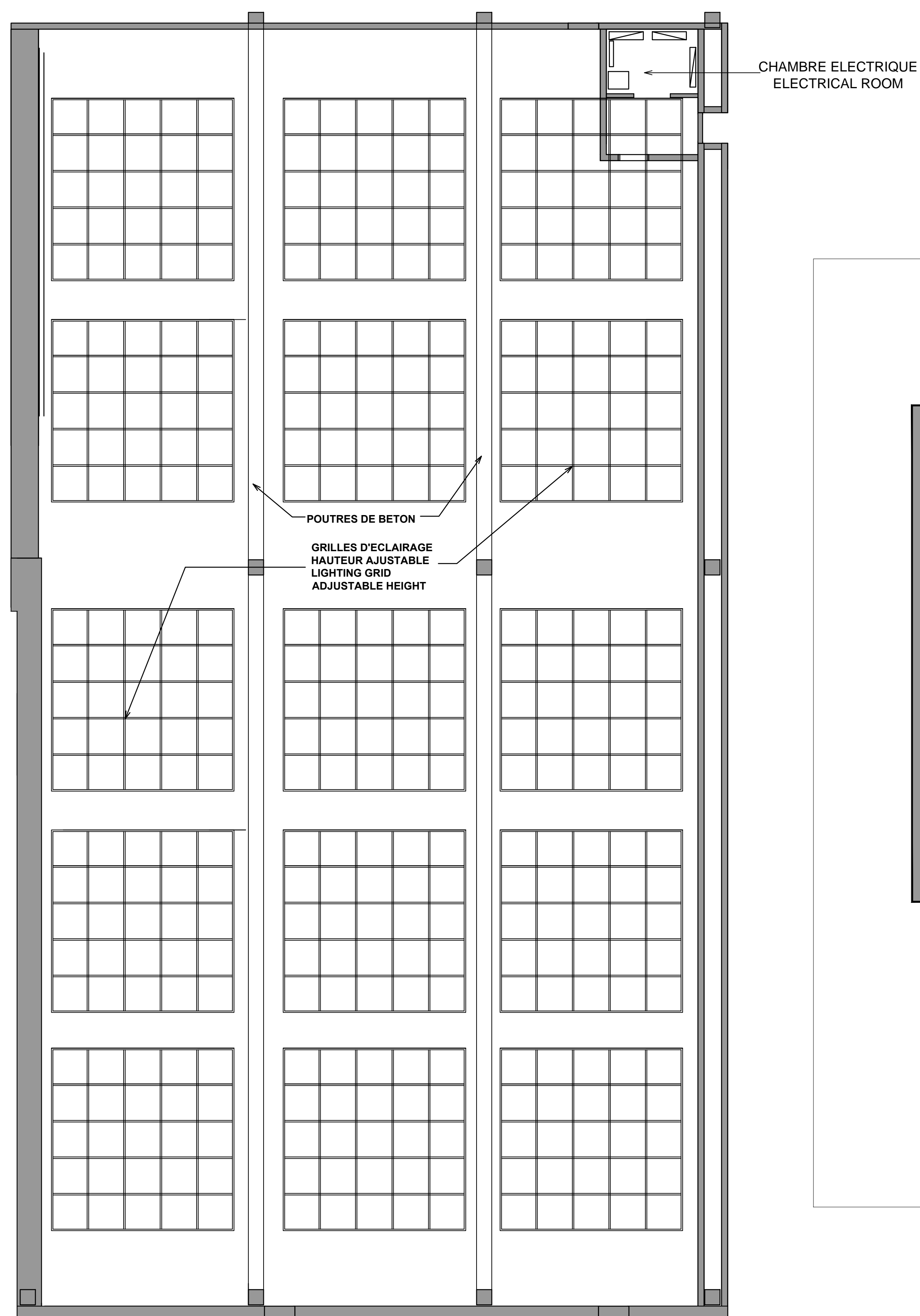
STUDIO A PLAN PLAFOND CEILING PLAN
