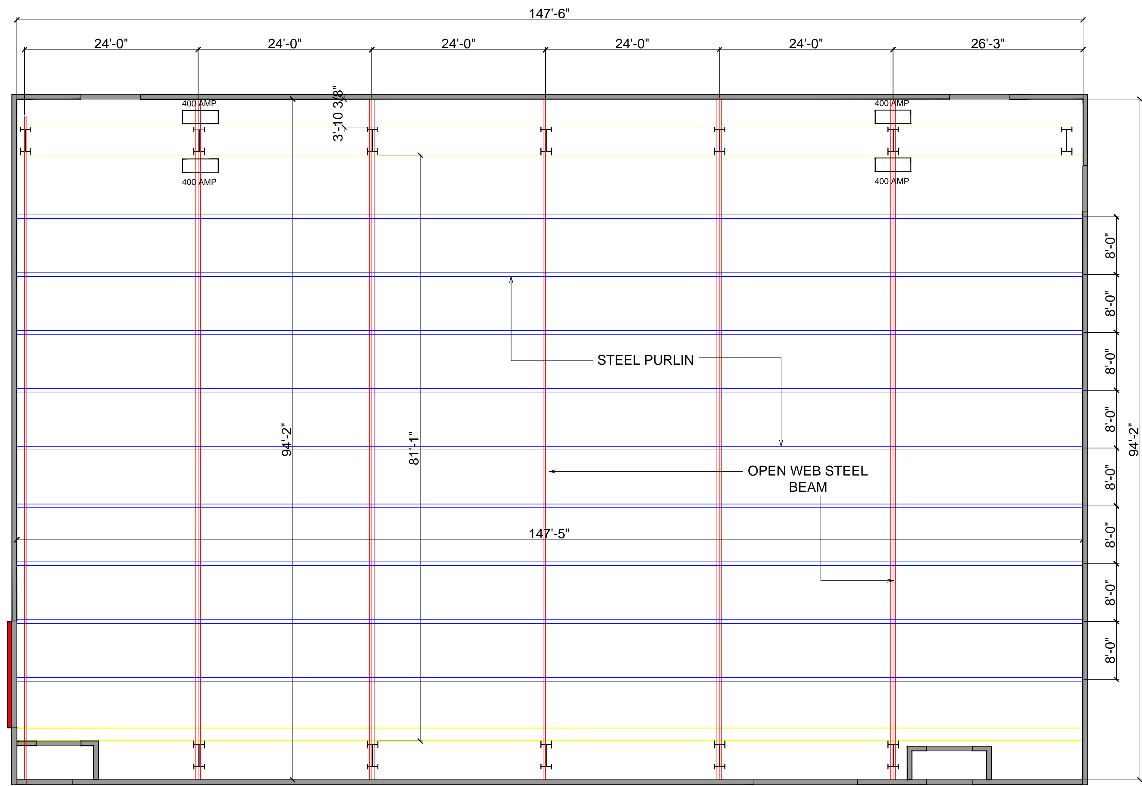
STUDIO CEILING PLAN
